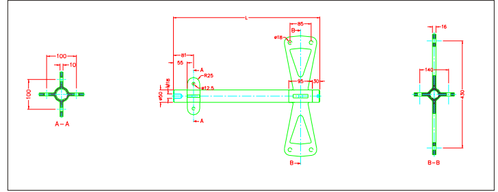
5542 拉桿支撐棒 Compression rod series for tension rod system
