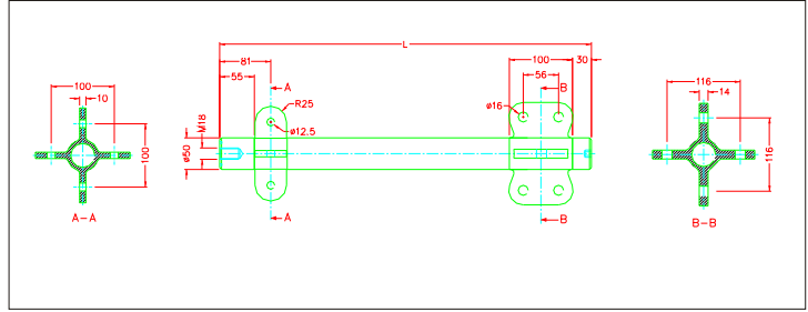
5531 拉桿支撐棒 Compression rod series for tension rod system
