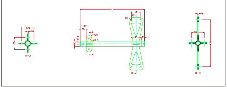
5541 拉桿支撐棒 Compression rod series for tension rod system
