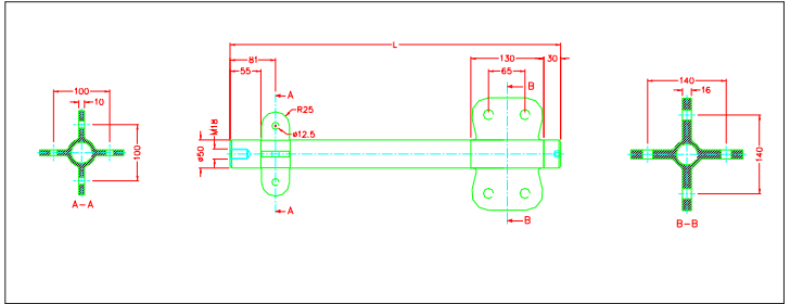
5532 拉桿支撐棒 Compression rod series for tension rod system
